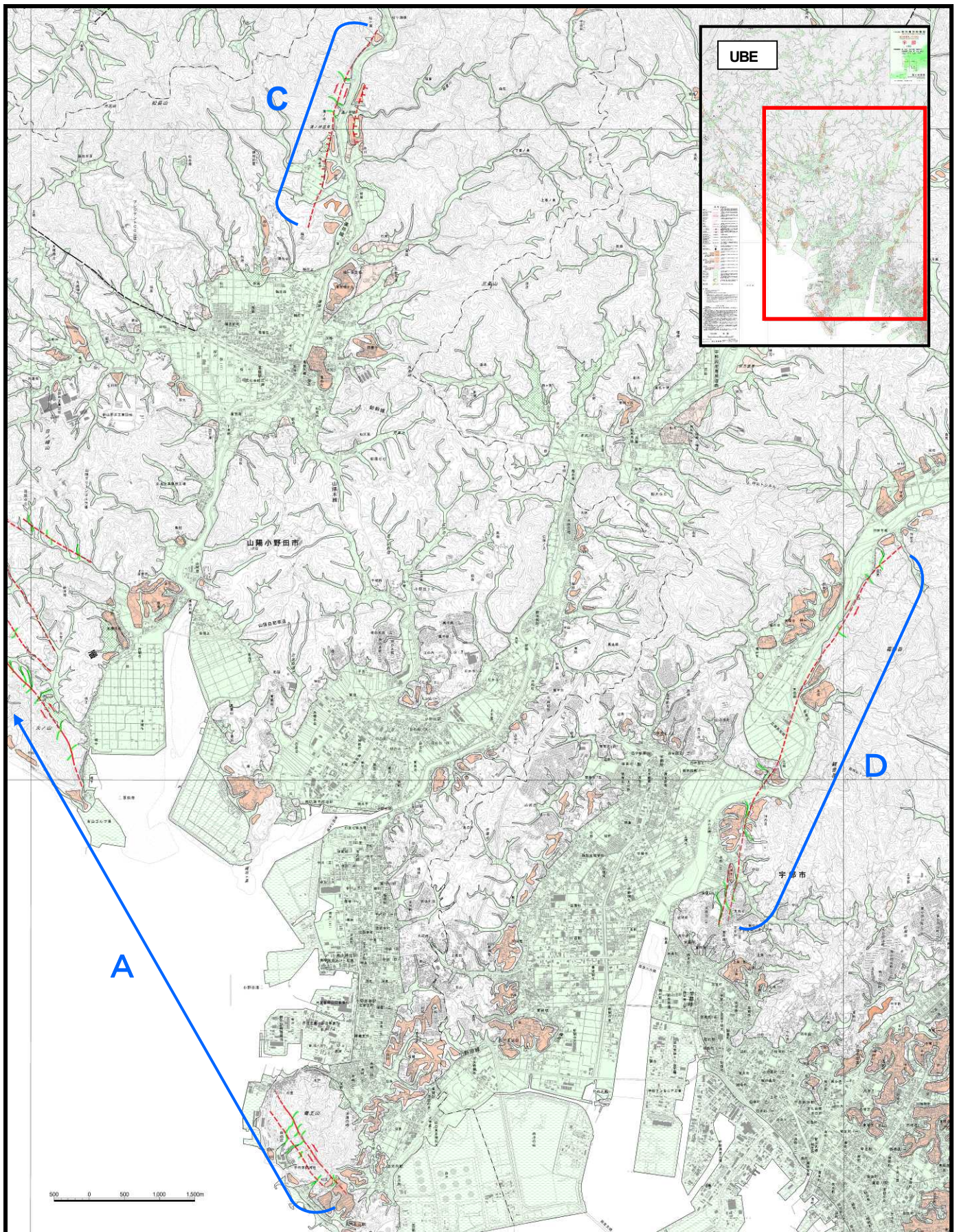
A: Kikugawa Fault C: Active Fault from Matsugase to kamonosho, Sanyo-Onoda City D: Active Fault from Jiseiji to Bunkyodai, UBE City
