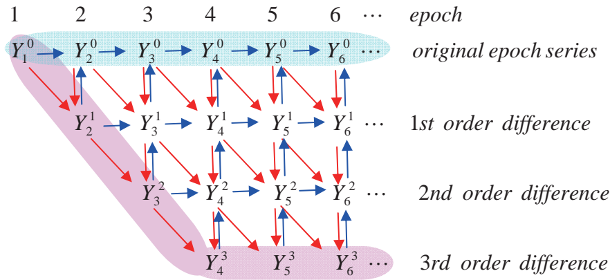
Fig. A-1 Schematic diagram of differential process (red arrows) and recovering process (blue arrows) for the case of M=3. The original epoch series and the processed one are hatched with light blue and magenta, respectively. The columns of the data elements in the diagram are regarded as “state vectors”.
